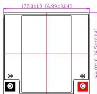
B2 Terminal
