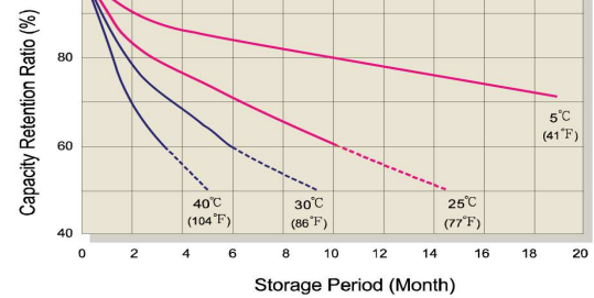
Capacity Retention Characteristic
